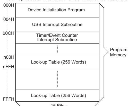
Program Memory
