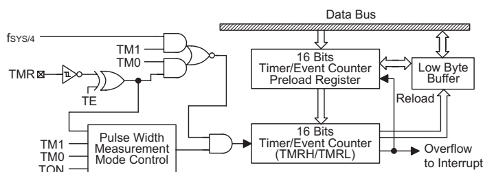
Timer/Event Counter
