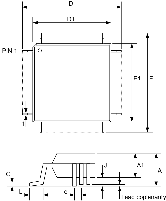
Figure 7 OX16PCI958 Package
