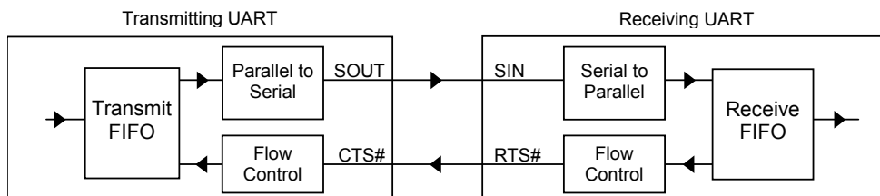
Figure 1 Auto Flow Control (Auto-RTS & Auto-CTS) Example
