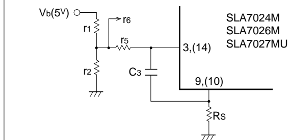
Fig. 3 Circuit for fixing the coil current
