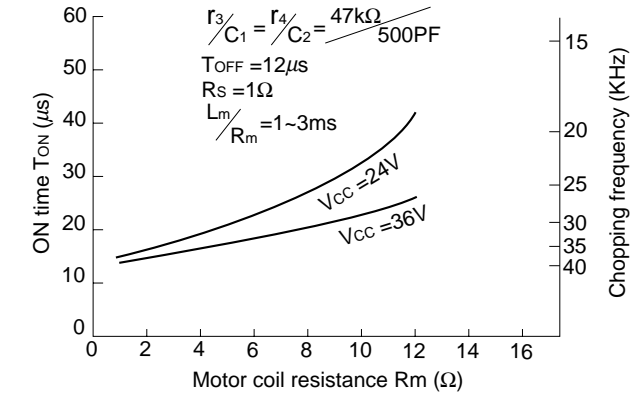
Fig. 10 Chopper frequency vs. Motor coil resistance
