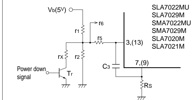
Fig. 5 Circuit for fixing the coil current
