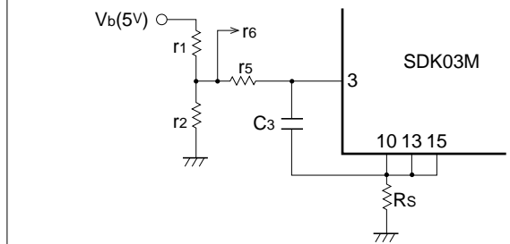
Fig. 4 Circuit for fixing the coil current
