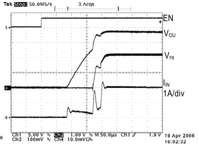
Start Up 1000mA Flash V_{IN}=3.6V , V_{OUT}=3.8V
