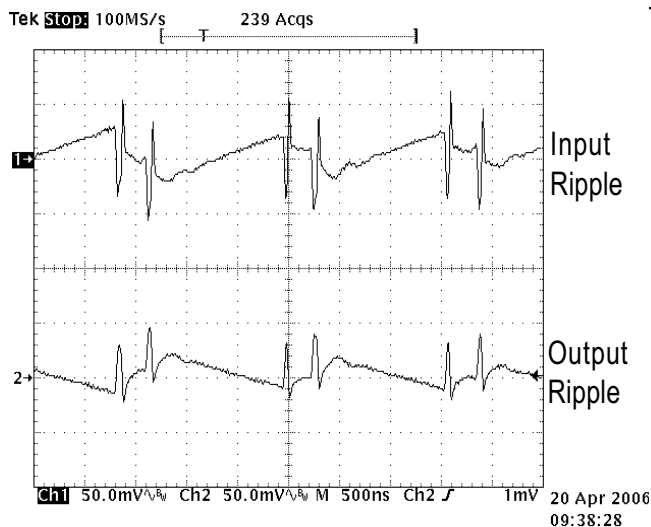
Ripple 1X Torch 200mA, V_{IN}=4.2V
