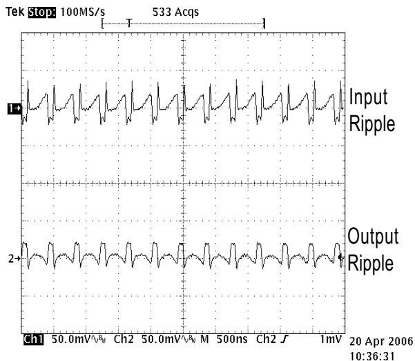
Ripple 1X Flash 700mA, V_{IN}=4.2V
