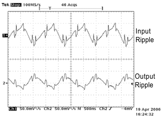
Ripple 1X Flash 1000mA, V_{IN}=4.2V
