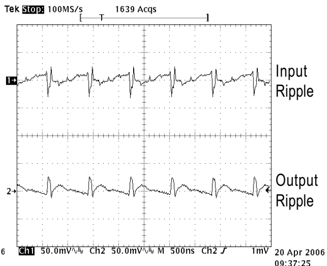
Ripple 2X Torch 200mA, V_{IN}=3.0V
