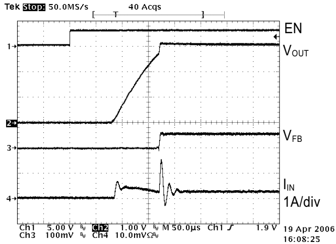
Start Up 200mA Torch V_{IN}=3.6V , V_{OUT}=3.1V
