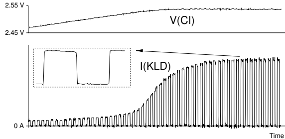
Figure 6: Turn-on behaviour, detailed view f(\text{IN}) = 100 \text{ kHz} (1:1), \text{CI} = 470 \text{ nF} , \text{RSET} = 10 \text{ k}\Omega
