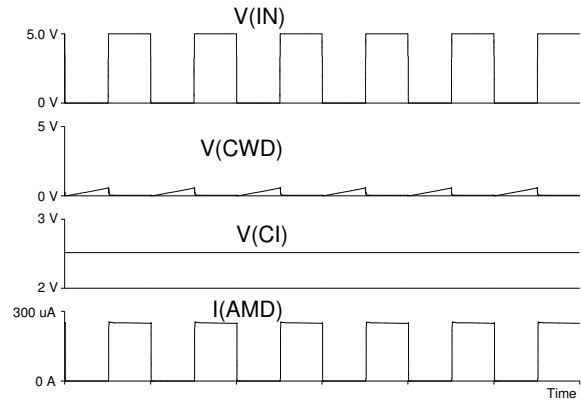
Figure 8: Watchdog, CWD open, f(\text{IN}) = 100 \text{ kHz} (1:1), \text{CI} = 470 \text{ nF} , \text{RSET} = 10 \text{ k}\Omega
