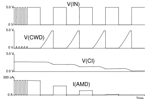
Figure 9: Watchdog, CWD open, f(\text{IN}) = 100 \text{ kHz} \rightarrow 10 \text{ kHz} (1:1), \text{CI} = 470 \text{ nF} , \text{RSET} = 10 \text{ k}\Omega
