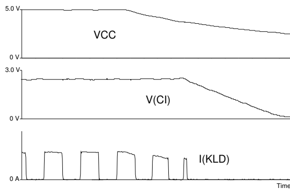
Figure 7: Turn-off behaviour, f(\text{IN}) = 100 \text{ kHz} (1:1), \text{CI} = 470 \text{ nF} , \text{RSET} = 10 \text{ k}\Omega
