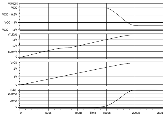
Figure 1: Turn-on behaviour
