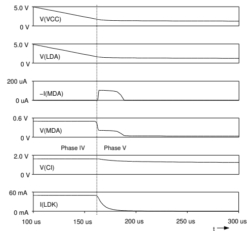
Figure 2: Turn-off behaviour
