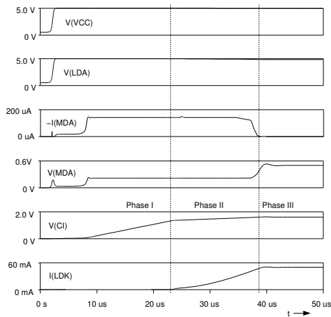
Figure 1: Turn-on behaviour
