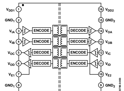
Figure 3. ADuM2402 Functional Block Diagram
