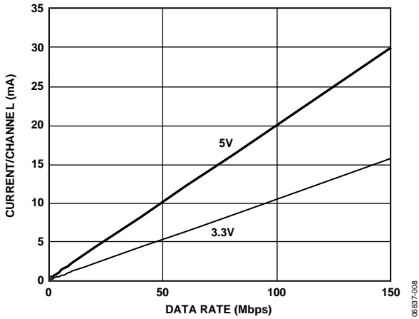
Figure 8. Typical Input Supply Current per Channel vs. Data Rate for 5 V and 3.3 V Operation
