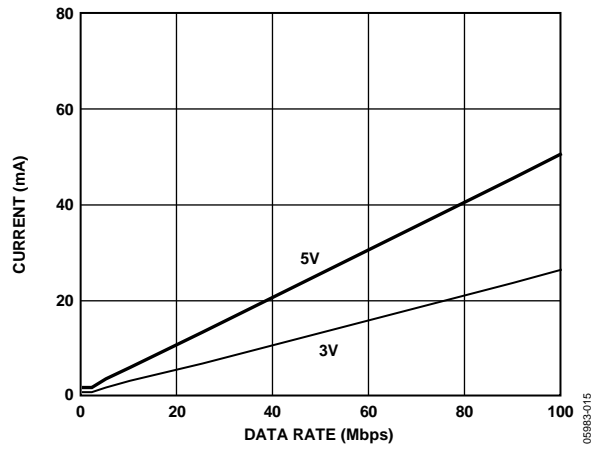
Figure 15. Typical ADuM3402 V_{DD1} or V_{DD2} Supply Current vs. Data Rate for 5 V and 3 V Operation
