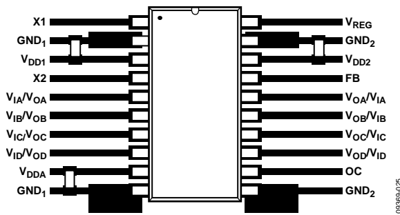
Figure 41. Recommended PCB Layout
