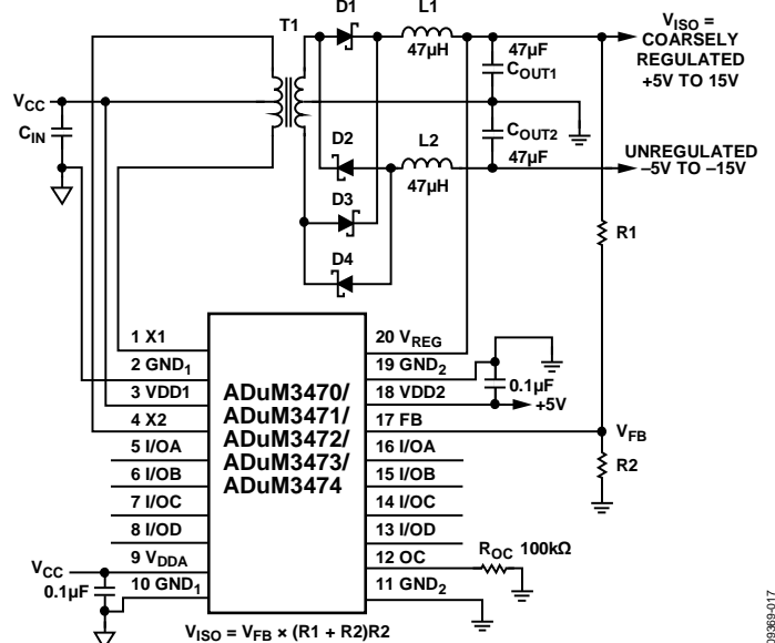
Figure 40. Positive and Unregulated Negative Supply
