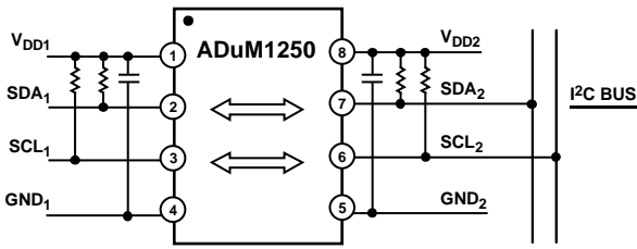
Figure 9. Typical Isolated I 2 C Interface Using ADuM1250
