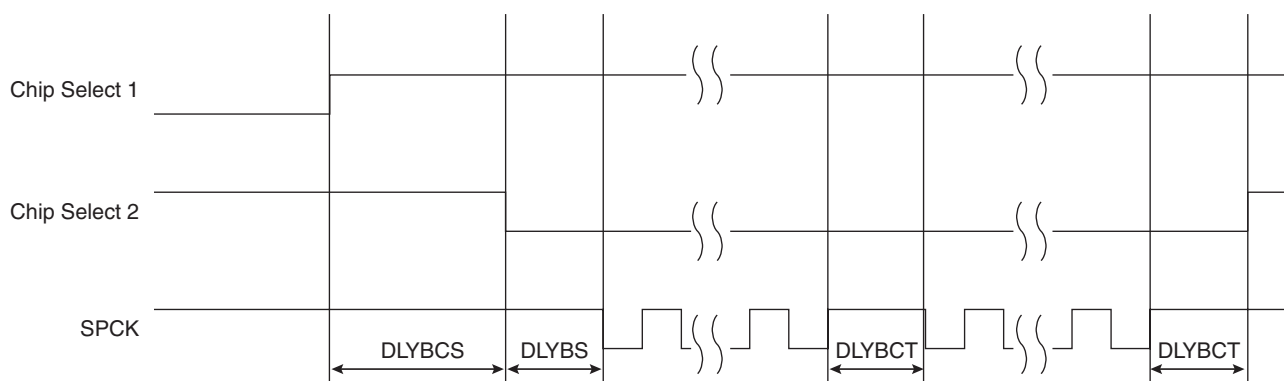
Figure 28-9. Programmable Delays
