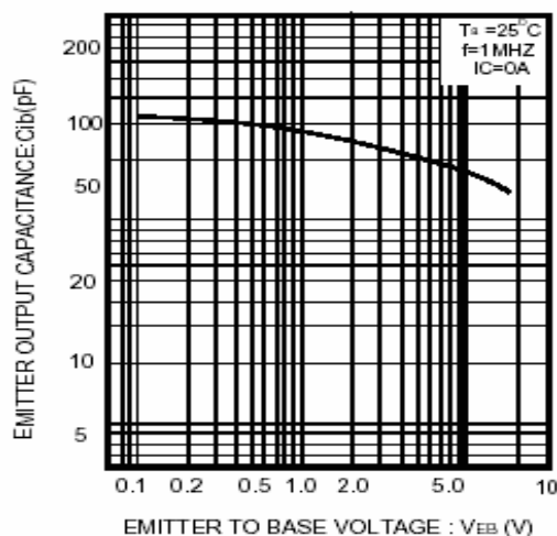
Fig.8 Emitter input capacitance vs emitter-base voltage
