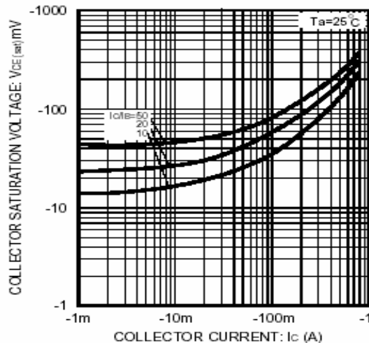
Fig.4 Collector-emitter saturation voltage vs. collector current (1)
