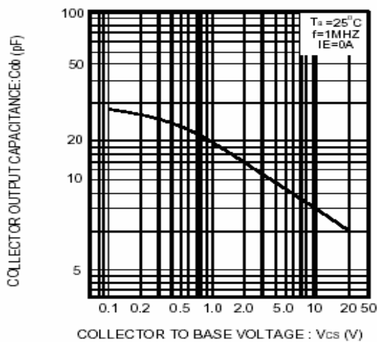
Fig.7 Collector output capacitance vs. collector-base voltage
