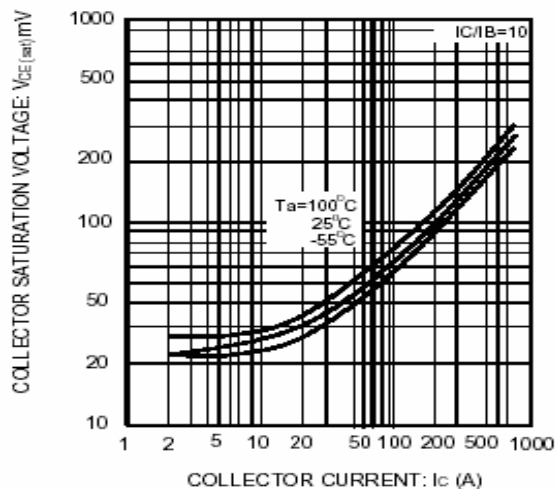
Fig.5 Collector-emitter saturation voltage vs. collector current (2)
