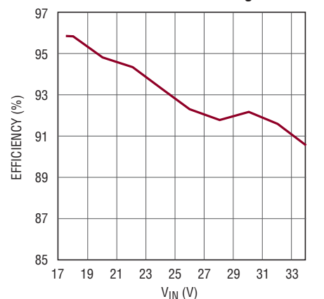
Efficiency vs V_{IN} , Buck Mode, 15.6V at 350mA LED String
