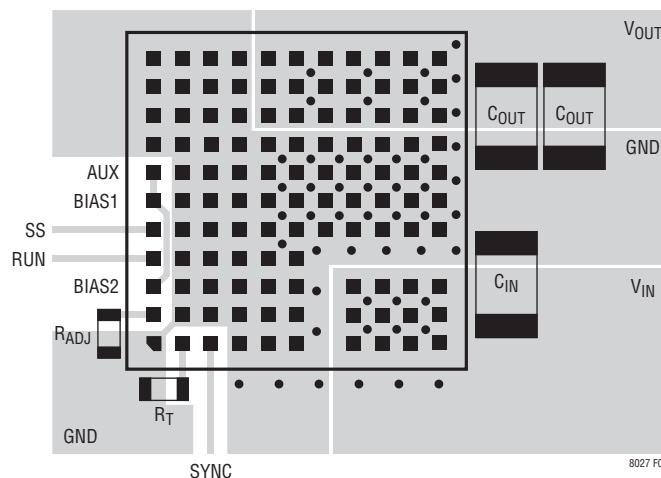
Figure 3. Suggested Layout
