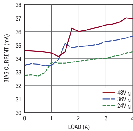
Bias Current vs Load, V_{OUT} = 15\text{V}
