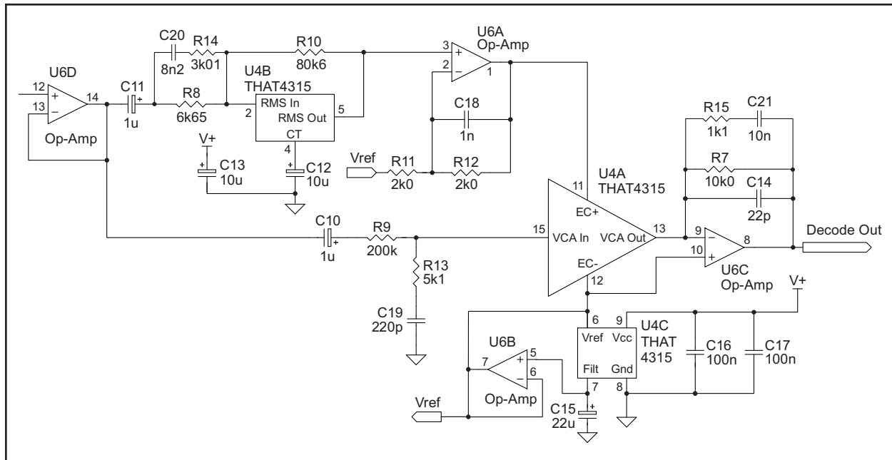
Figure 9. 3:1 Decoder circuit
