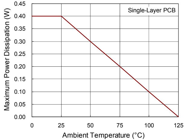
Figure 3. Derating Curves for RT8060A Package
