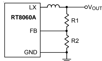
Figure 1. Output Voltage Setting
