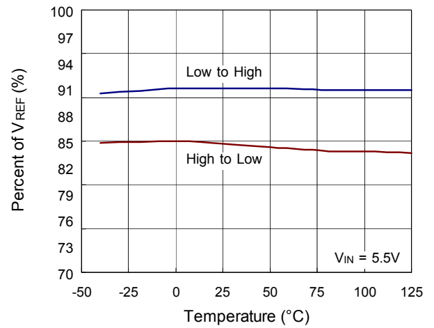
PGOOD Threshold vs. Temperature
