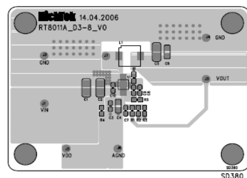
Figure 8. RT8011A Demo Board (Only WDFN-8E 3x3)
