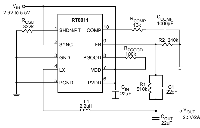
Figure 1. Typical Application Circuit for RT8011
