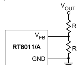
Figure 6. Setting the Output Voltage
