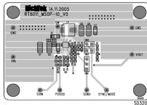
Figure 7. RT8011 Demo Board
