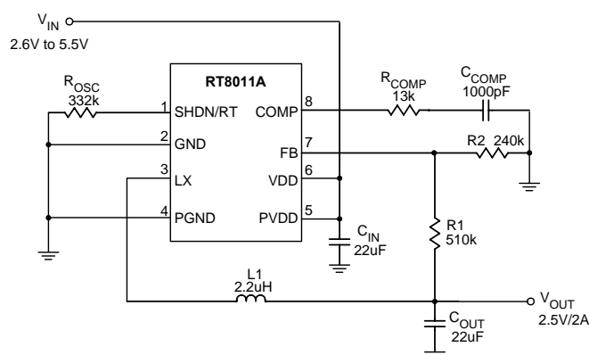
Figure 2. Typical Application Circuit for RT8011A
