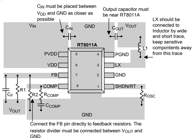
Figure 4. RT8011A Layout Guide
