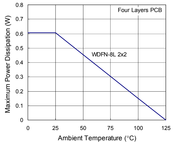
Figure 5. Derating Curves for RT8010B Package
