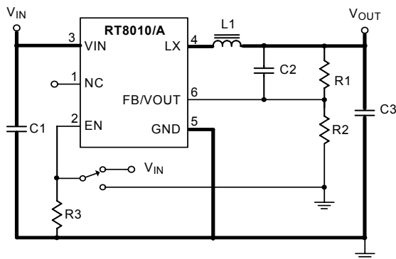
Figure 6. EVB Schematic
