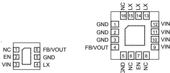
WDFN-6L 2x2 (RT8010)
