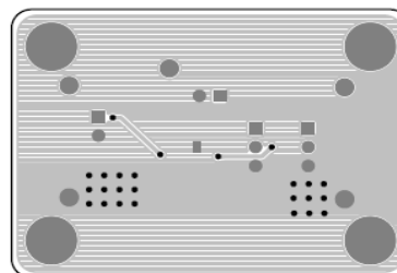
Figure 8. Bottom Layer
