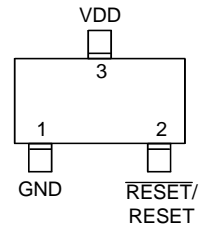
SOT-23-3 (L-Type)
