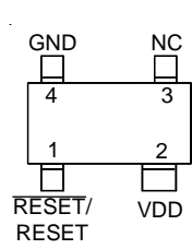
SC-82
