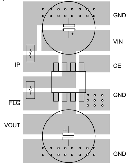
Board Layout
