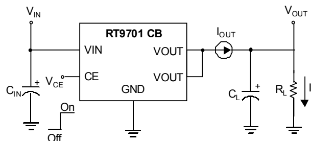
Test Circuit 3
