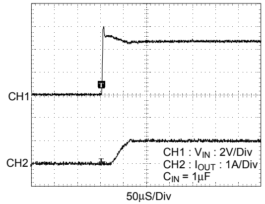
Soft-start Short Circuit Response
