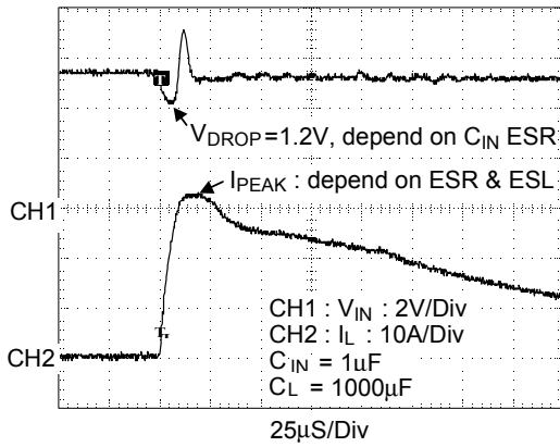
Inrush Short Circuit Response
