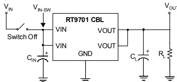
Test Circuit 2
