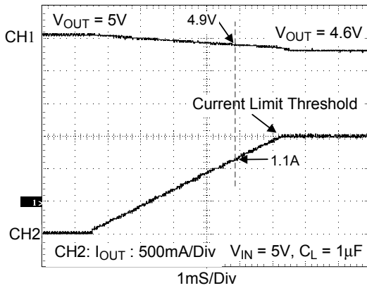
Ramped Load Response
