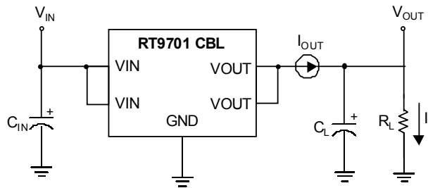
Test Circuit 1
