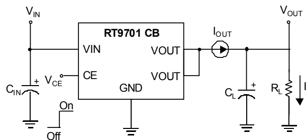
Test Circuit 3
