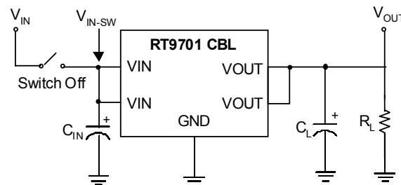
Test Circuit 2
