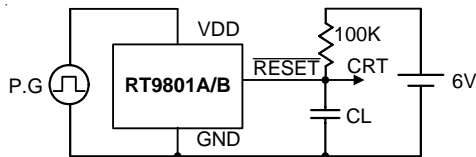
Dynamic Response
