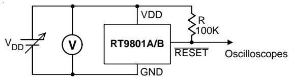
Detection Voltage
