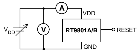
Current Consumption
