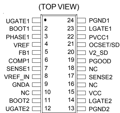
TSSOP-24 & SOP-24
