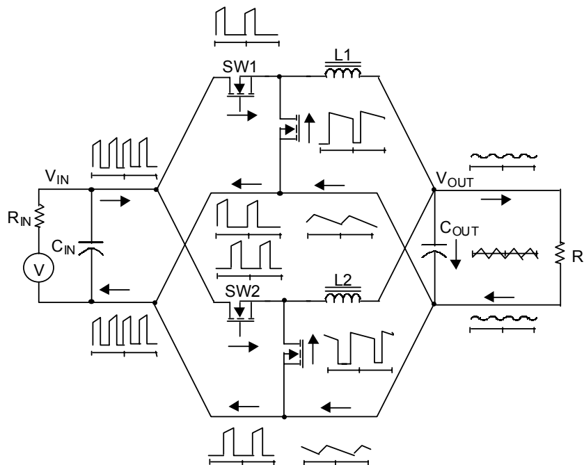
Fig.7 Power Stage Ripple Current Path
