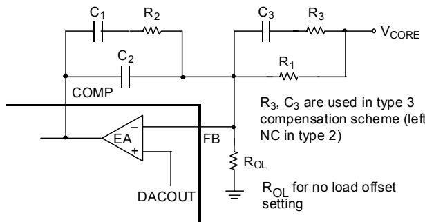
Fig. 5 EA Compensation Network
