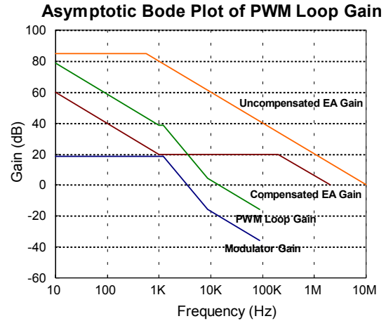
Fig. 6 Asymptotic Bode Plot of PWM Loop Gain
