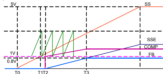
Figure 1. Timing diagram of softstart
