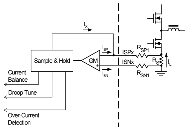
Figure 1. Current Sense Circuit
