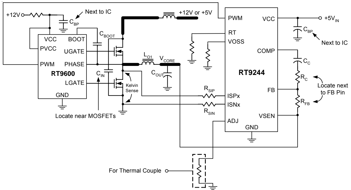
Figure 8. Layout Consideration
