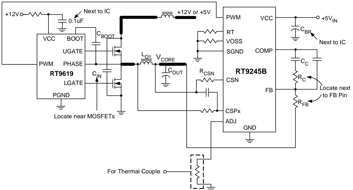
Figure 33. Layout Consideration
