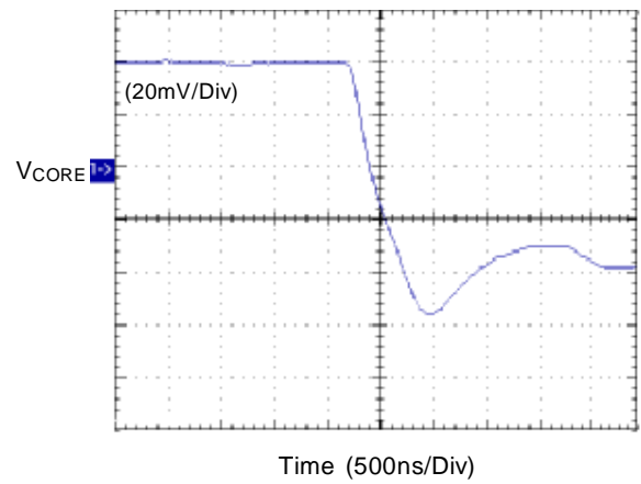
Transient Falling
