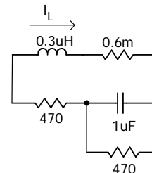
Figure 10. GM4 Setting for current ratio function
