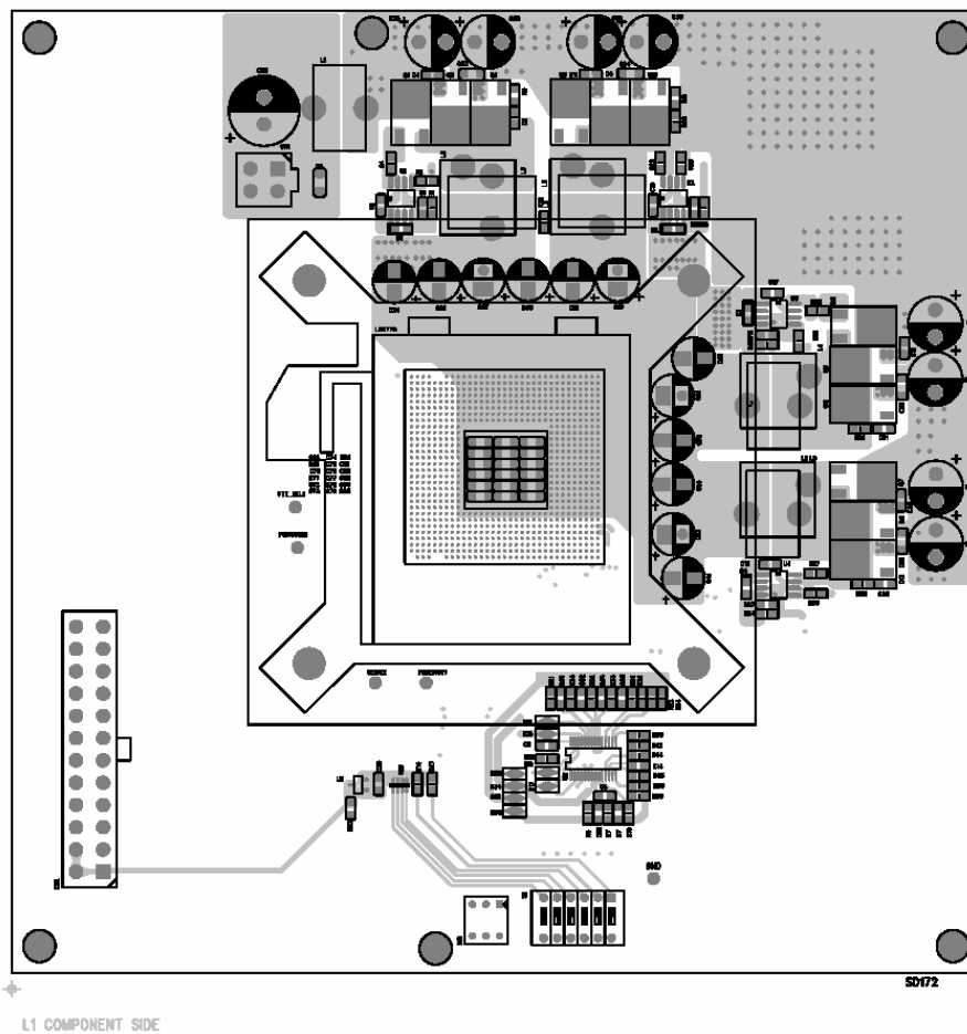
Figure 34. Layout of power stage
