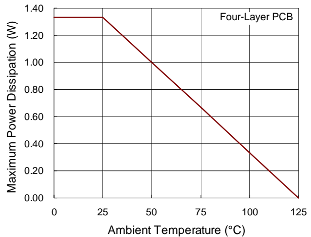
Figure 6. Derating Curves for RT8288A Package
