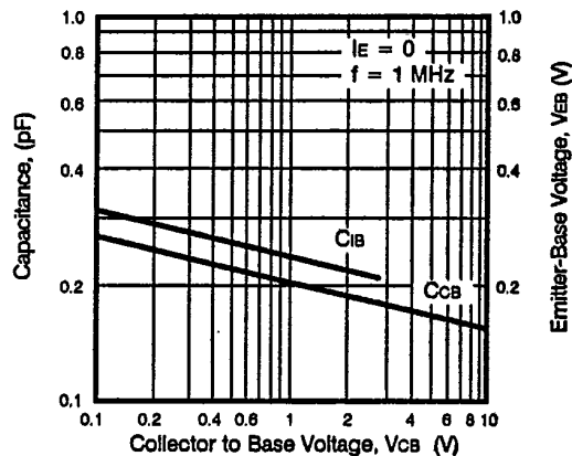
DEVICE CAPACITANCE
