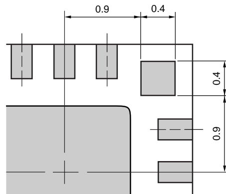
Dimensions of pin No.1 indication
