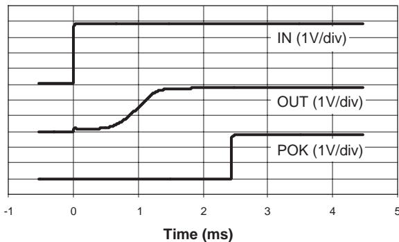
Power-Up With 100mA Load
