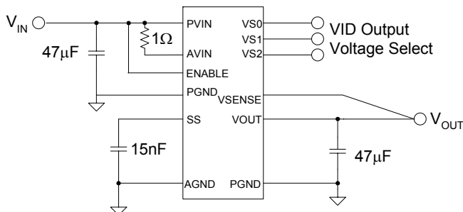
Figure 1. Simple Layout.
