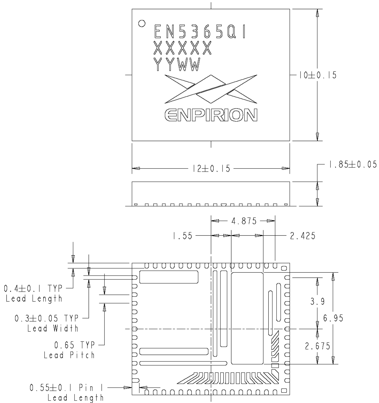
Figure 9. Package dimensions.
