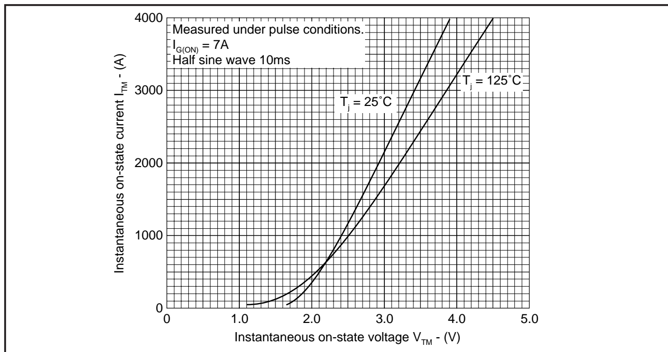
Fig.2 On-state characteristics
