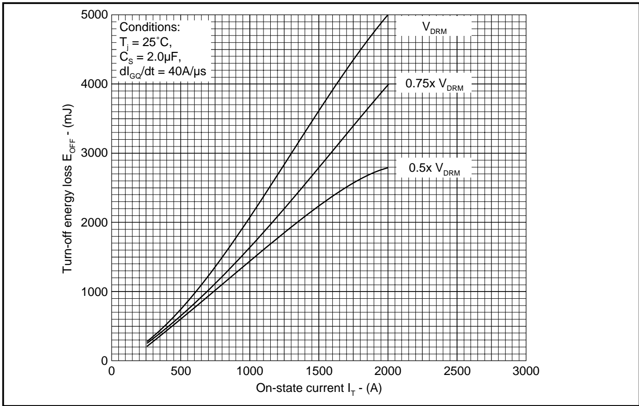
Fig.15 Turn-off energy vs on-state current
