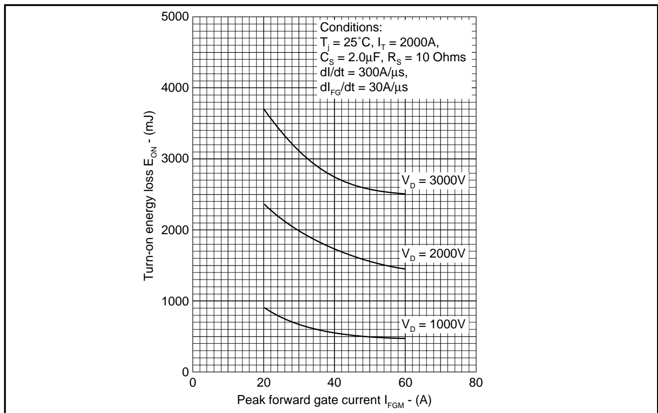
Fig.9 Turn-on energy vs peak forward gate current
