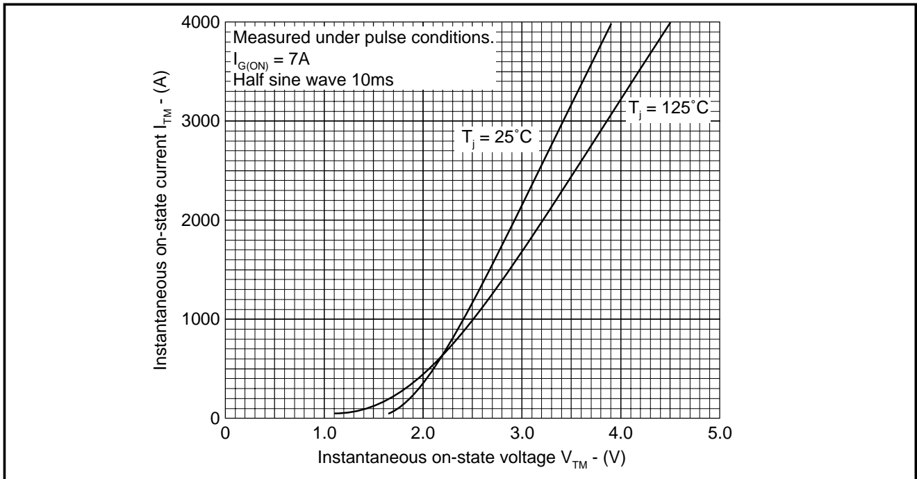
Fig.2 On-state characteristics
