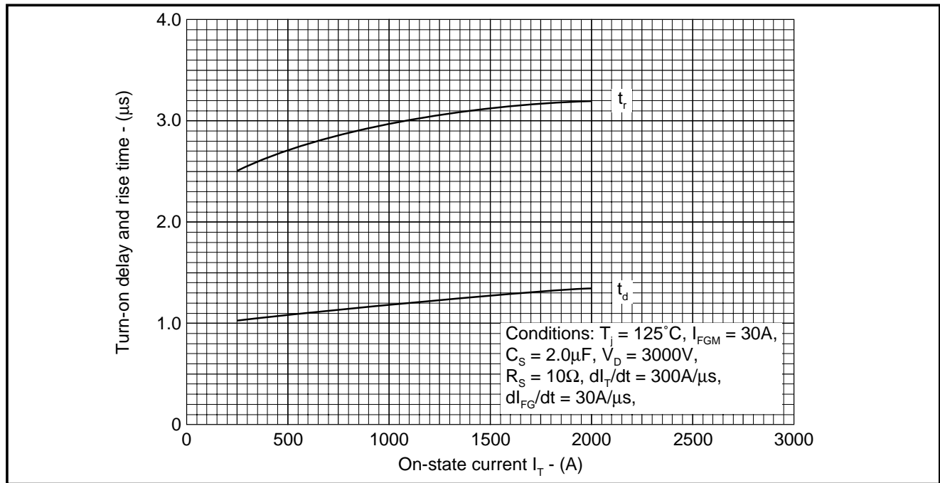
Fig.13 Delay time & rise time vs turn-on current
