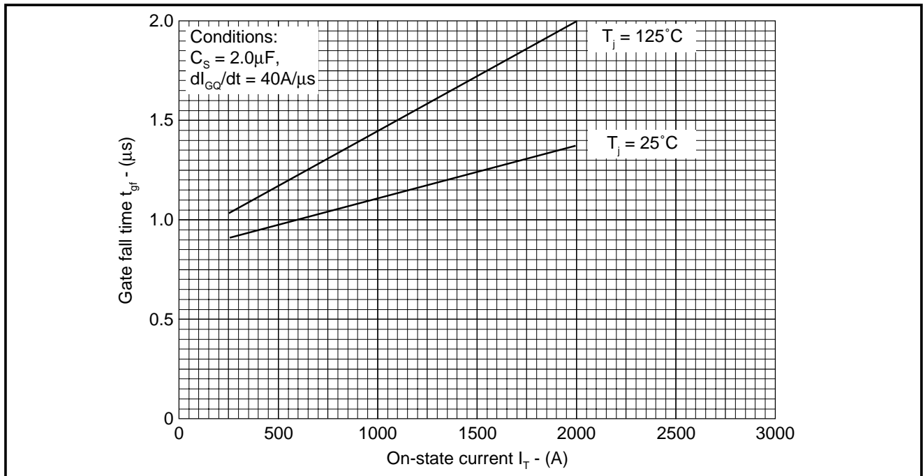
Fig.22 Gate fall time vs on-state current
