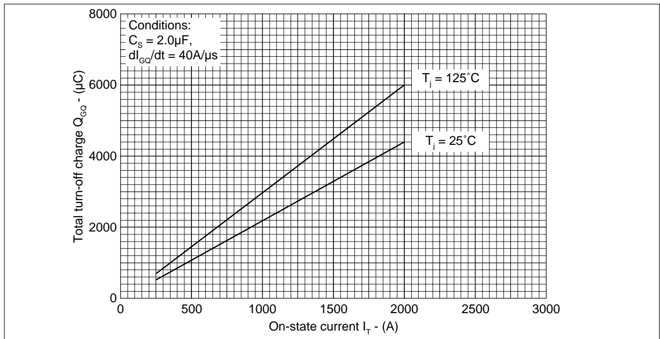
Fig.26 Turn-off gate charge vs on-state current
