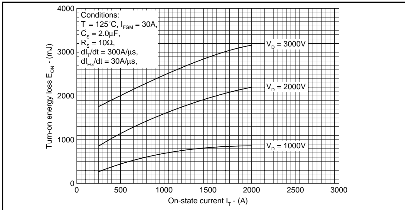
Fig.10 Turn-on energy vs on-state current
