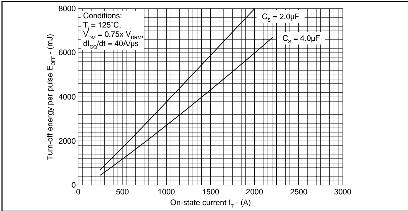
Fig.19 Turn-off energy vs on-state current
