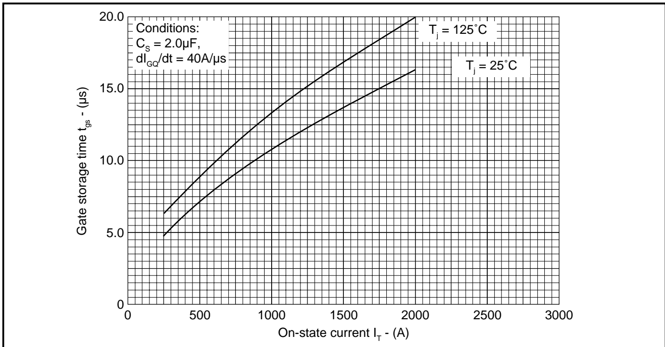
Fig.20 Gate storage time vs on-state current
