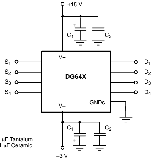
FIGURE 7. Supply Decoupling
