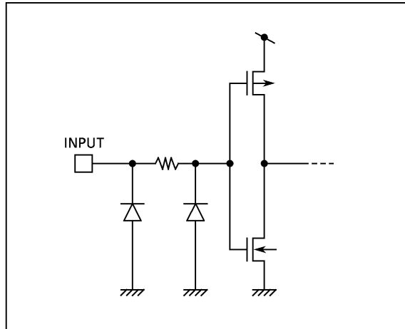
Input Equivalent Circuit
