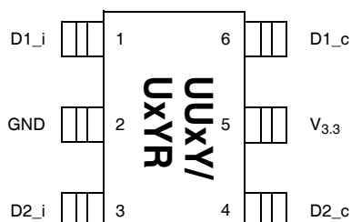
6-pin SOT23
