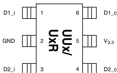
6-pin SC70
