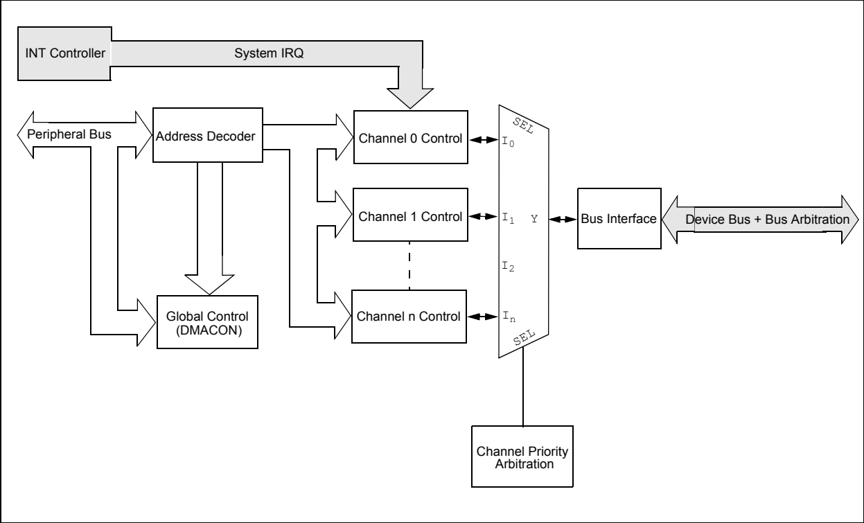
FIGURE 5-1: DMA CONTROLLER BLOCK DIAGRAM
