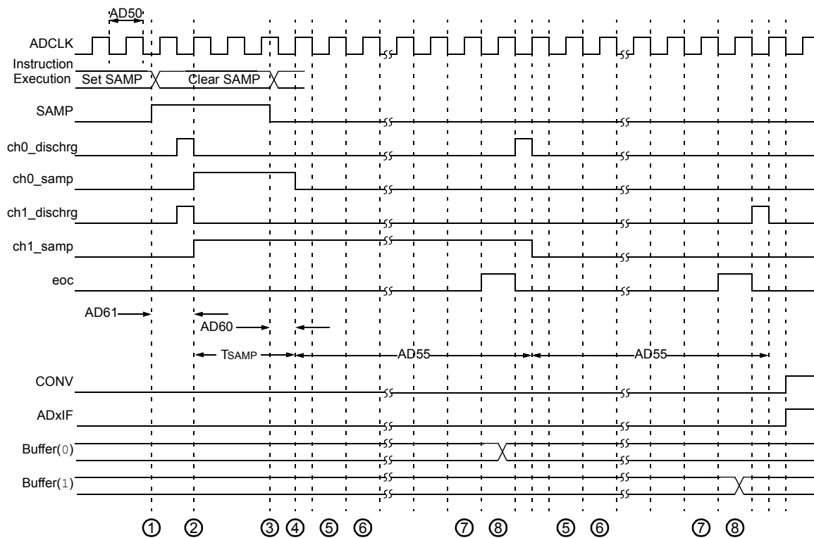
FIGURE 29-17: A/D CONVERSION (10-BIT MODE) TIMING CHARACTERISTICS (CHPS<1:0> = 01, SIMSAM = 0, ASAM = 0, SSRC<2:0> = 000)
