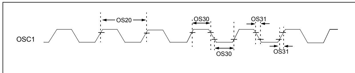
FIGURE 29-2: EXTERNAL CLOCK TIMING
