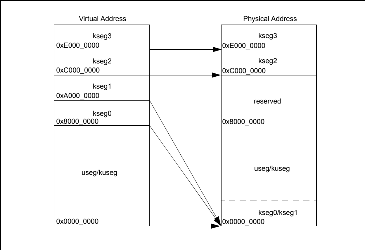
FIGURE 2-5: PIC32MX CORE FMT MEMORY MAP (ERL = 1)
