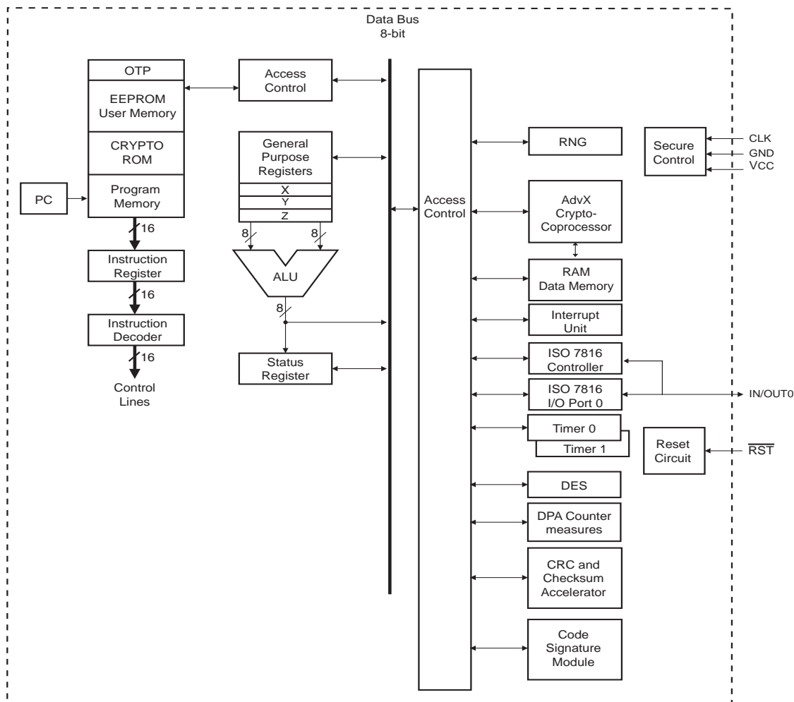
Figure 1. AT90SC28848RCU SecureAVR Enhanced RISC Architecture
