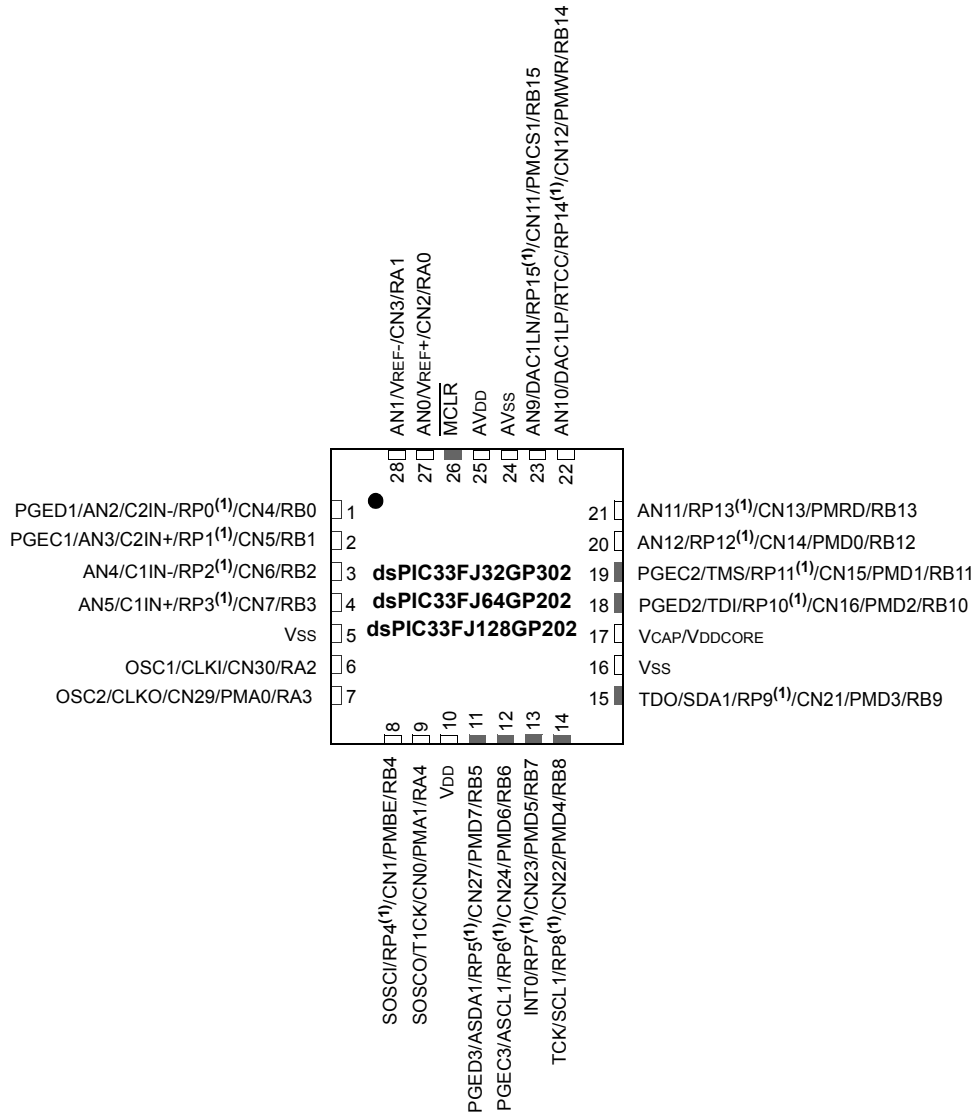
28-Pin QFN-S (2)
