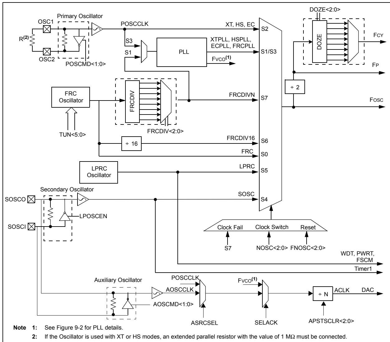
FIGURE 9-1: dsPIC33FJ32GP302/304, dsPIC33FJ64GPX02/X04 AND dsPIC33FJ128GPX02/X04 OSCILLATOR SYSTEM DIAGRAM
