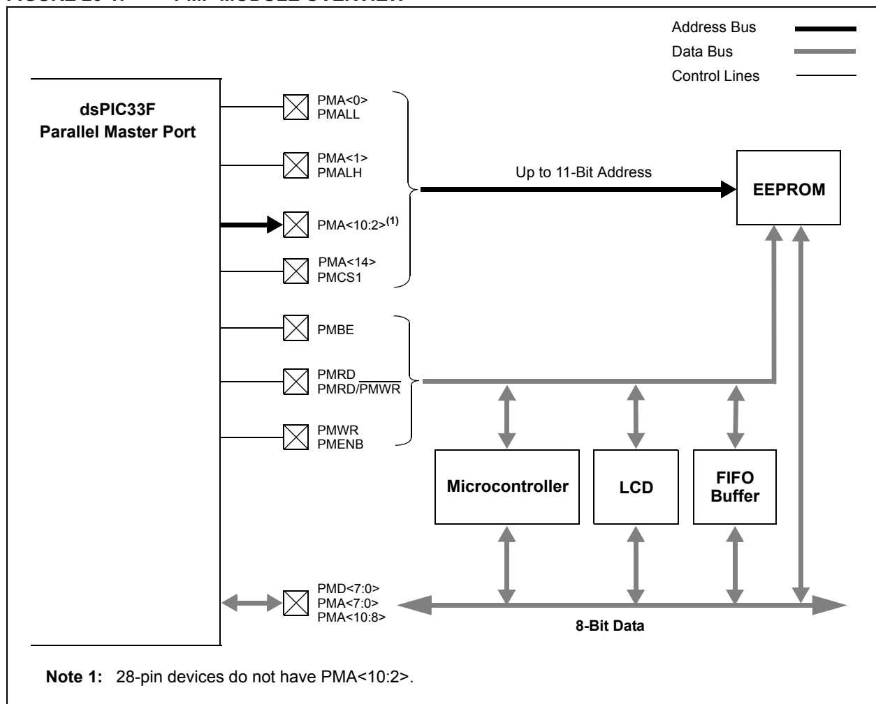
FIGURE 26-1: PMP MODULE OVERVIEW
