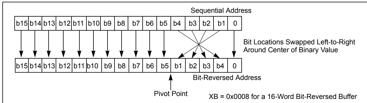
FIGURE 4-8: BIT-REVERSED ADDRESS EXAMPLE
