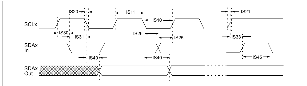
FIGURE 30-16: I2Cx BUS DATA TIMING CHARACTERISTICS (SLAVE MODE)
