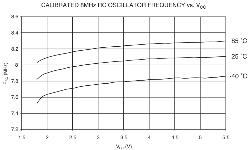
Figure 29-47. Calibrated 8 MHz RC Oscillator Frequency vs. V_{CC}
