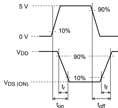
(c) V_{OUT}
