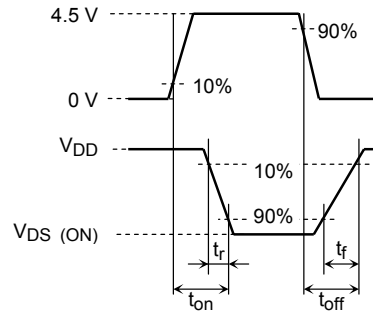
(c) V_{OUT}
