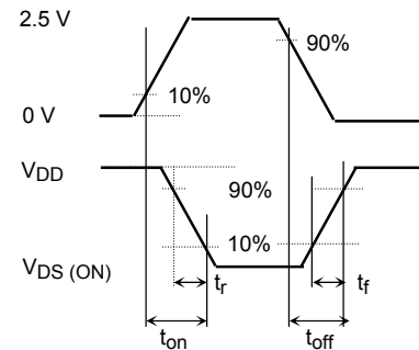
(c) V_{OUT}
