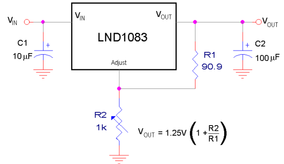
1.2V to 15V adjustable regulator
