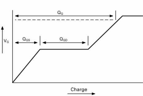
Basic gate charge waveform
