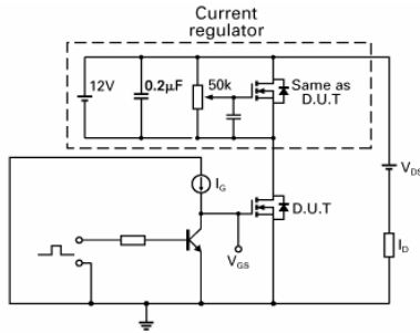
Gate charge test circuit
